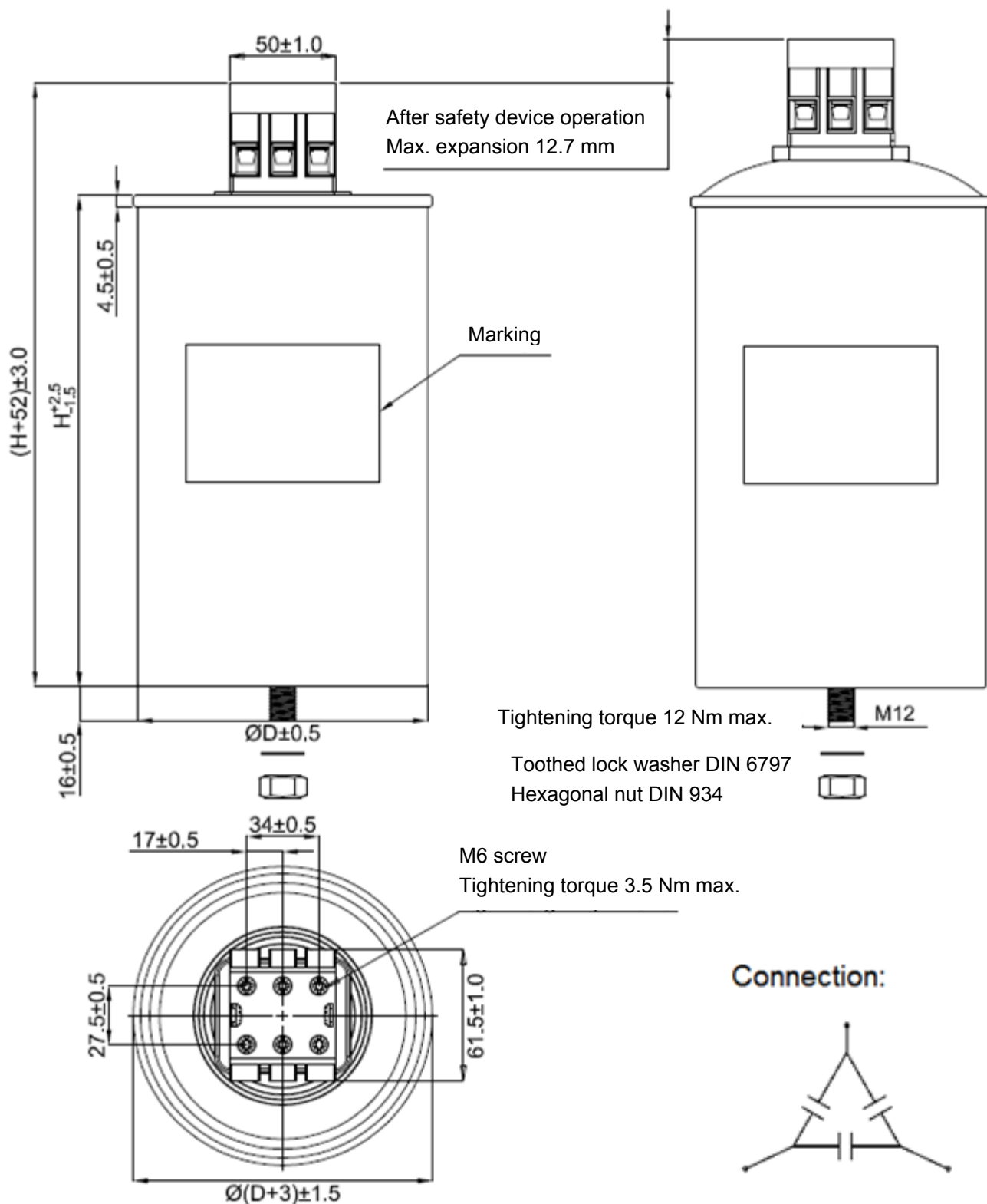
B32377: Delta connection type C
