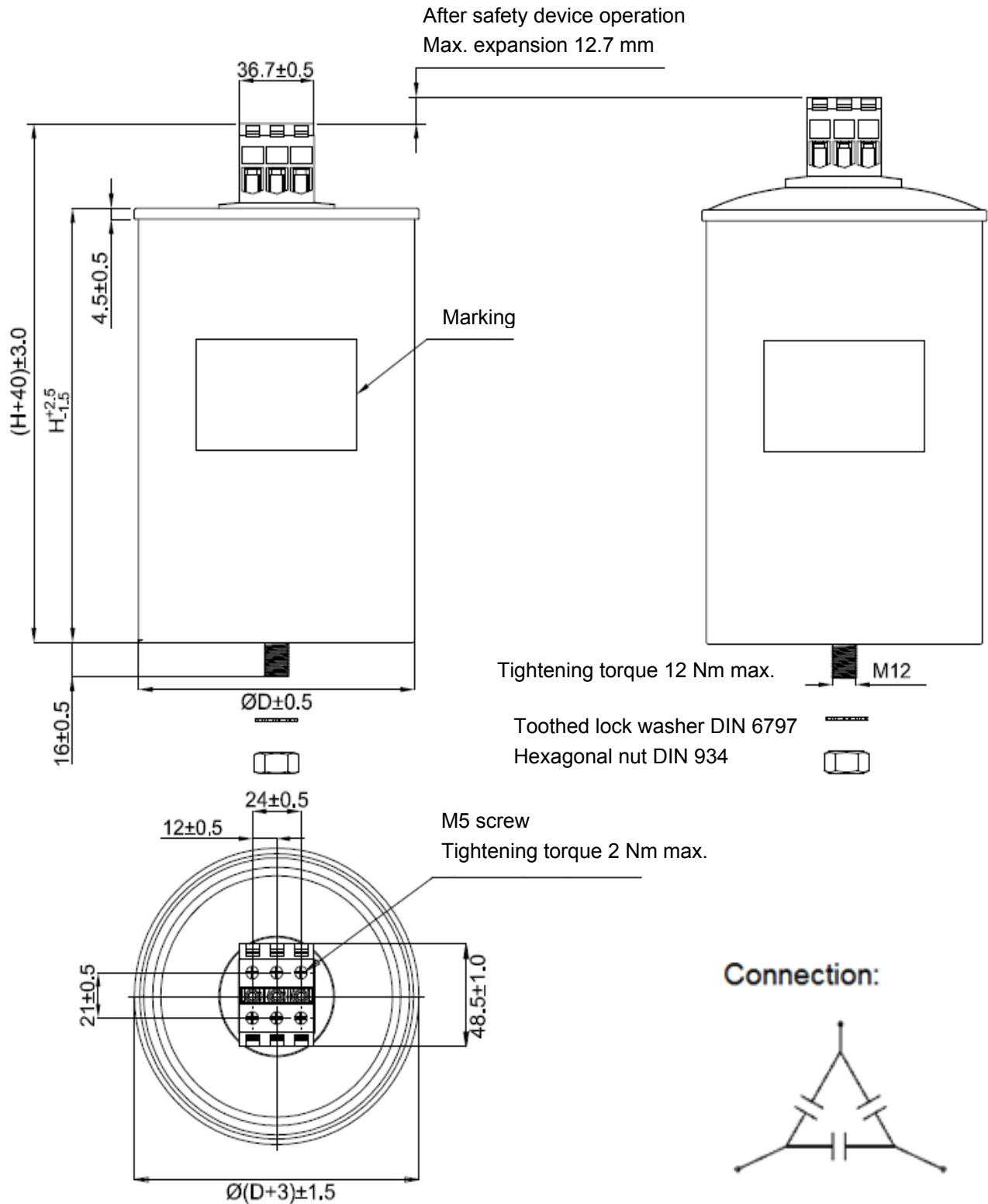
B32377: Delta connection type B
