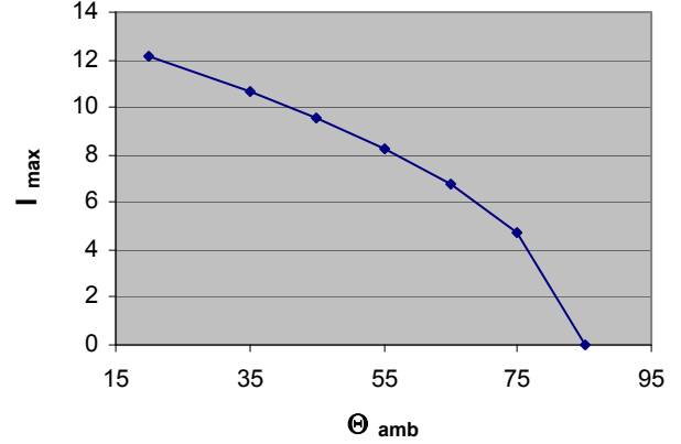
Max. allowable current (rms) at specific ambient Temp. B32344E4071A540
